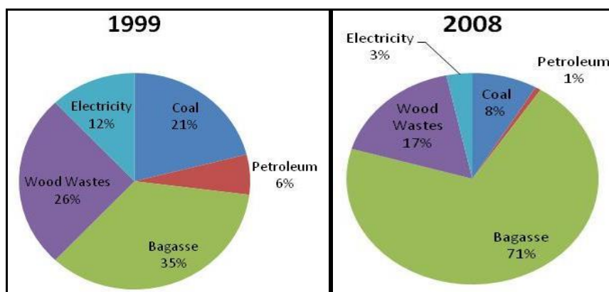
Figure 48 Industry energy consumption
