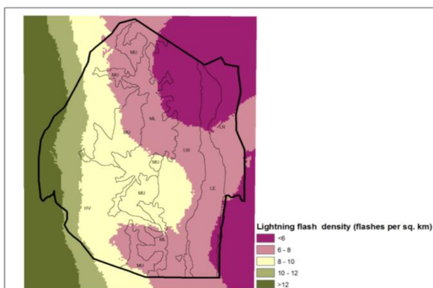
Figure 26 Spatial distribution of average lightning flash density in Swaziland, 2006-2010
