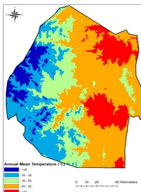
Figure 23 Distribution of mean annual temperature
