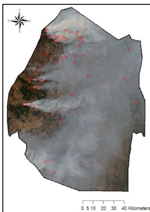
Figure 27 Satellite image showing extent of smoke from wildfires
