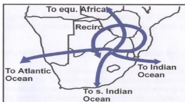
Figure 17 Transport pathways out of the South African Highveld
